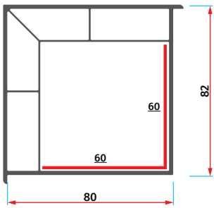
AMS 8012 Kutu Profili 80x80 Box Profile 80x80
