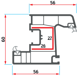
AMS 6020 3 Odacık Pencere Kanat Profili Economic Window Sash Profile
