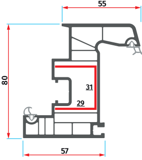
AMS 8003 Pencere Kanat Profili Window Sash Profile
