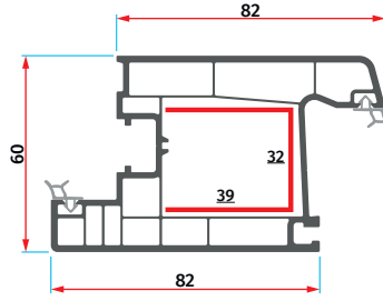
AMS 6021 3 Odacık Kapı Kanat Profili Economic Door Sash Profile
