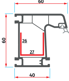
AMS 6018 3 Odacık Kasa Profili Economic Frame Profile
